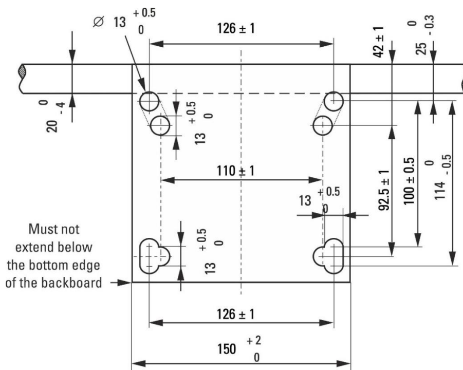
Diagram 7 Ring mounting plate for existing baskets (example dimensions)
